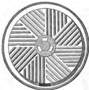
THE NETHER MILLSTONE.
